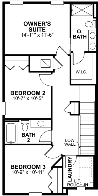
SECOND FLOOR
